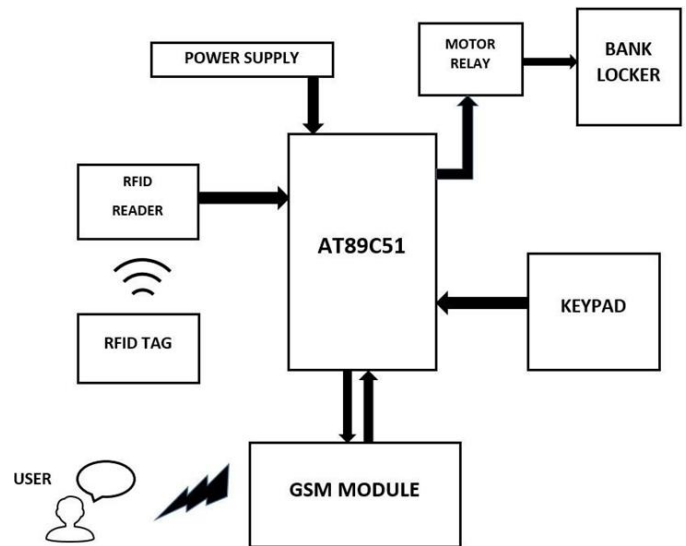
Fig1. Block diagram of bank locker system
